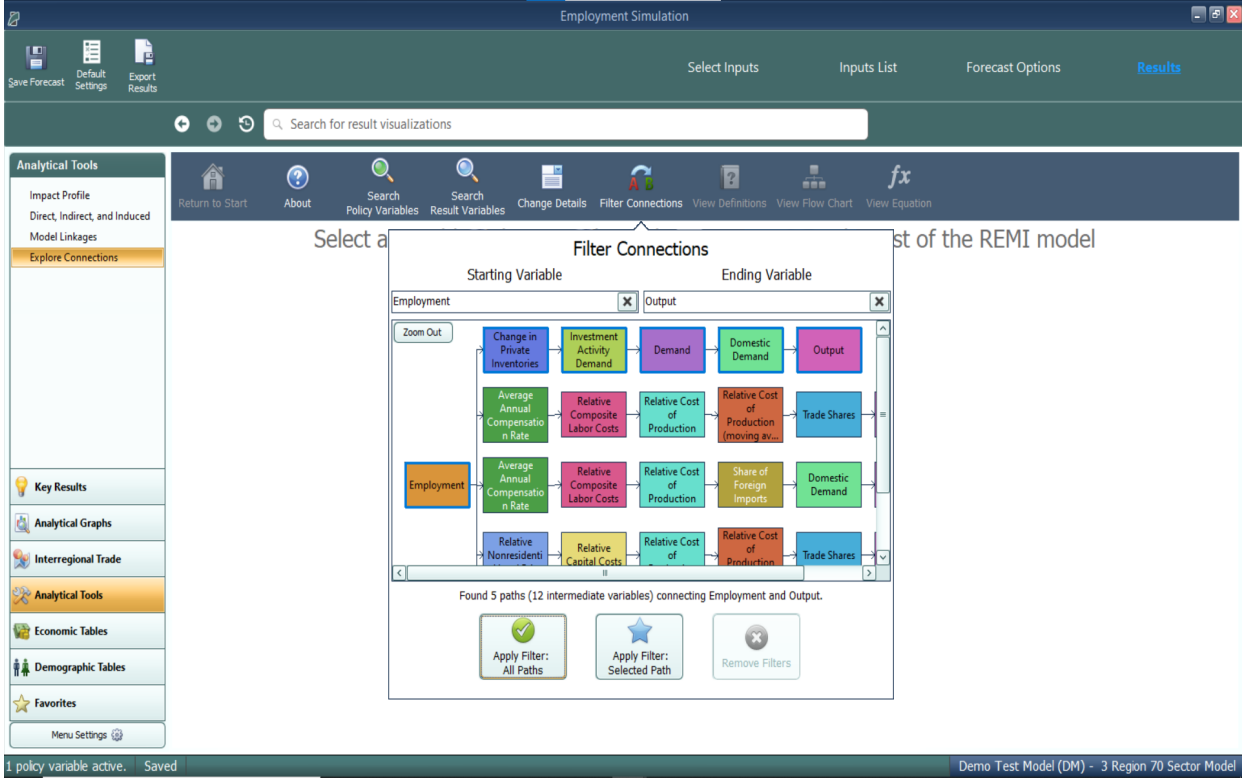
Figure 74: Connections Filter
