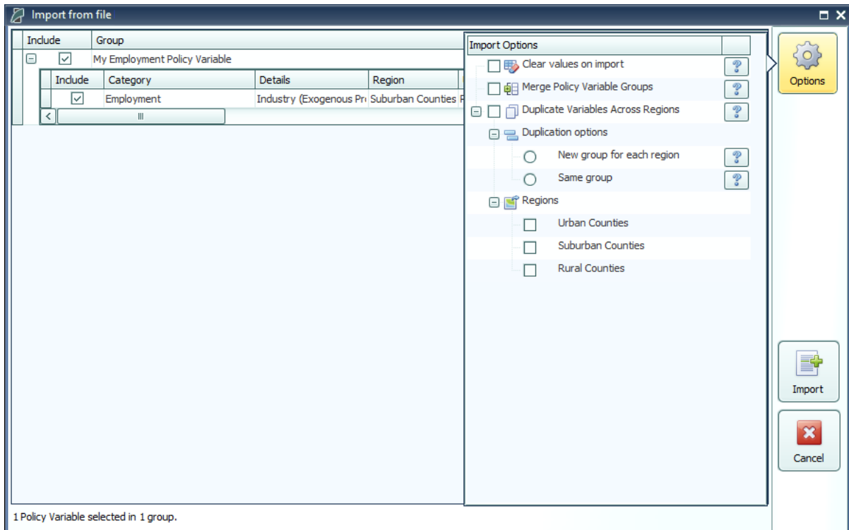
Figure 50: Import Center
