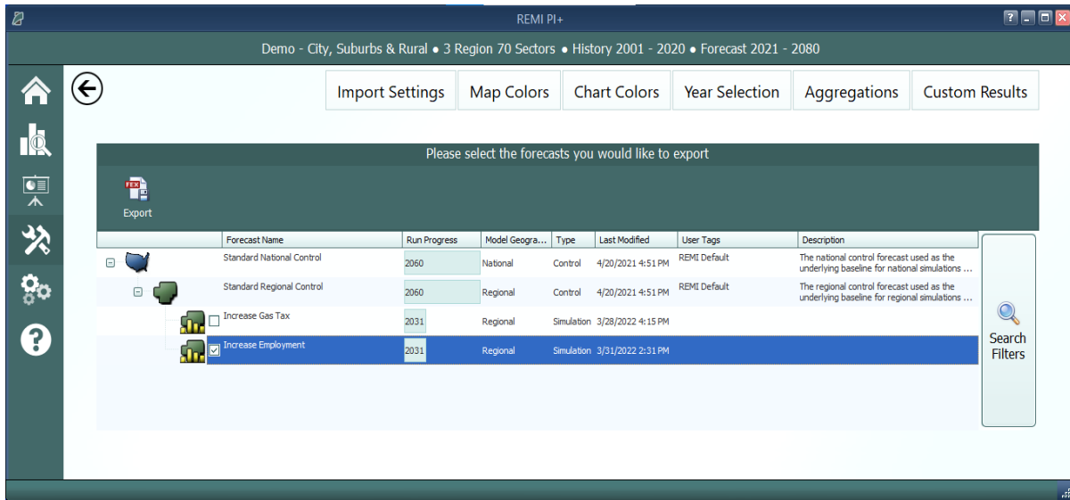
Figure 14: Forecast Export
