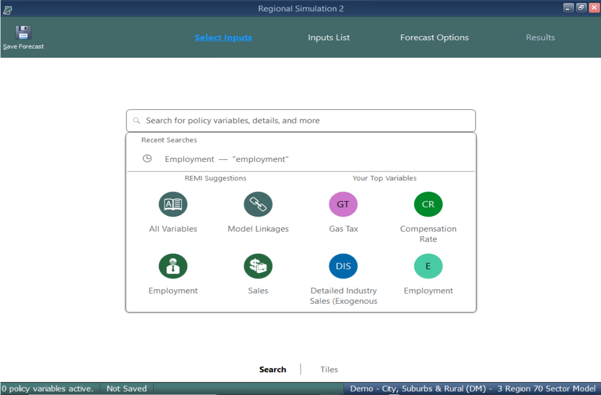
Figure 33: Forecast Window
