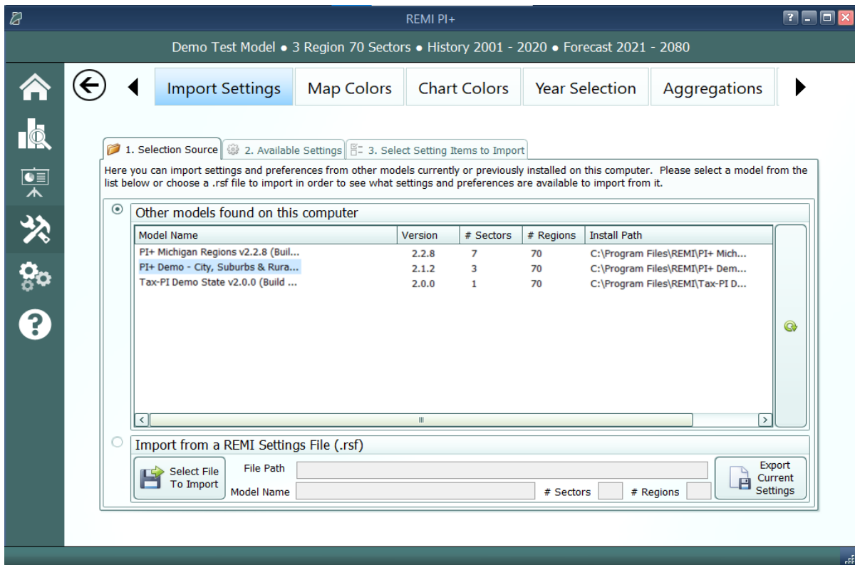
Figure 16: Import Manager
