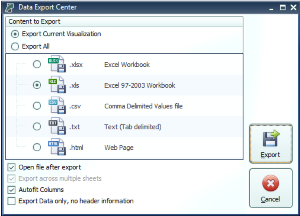
Figure 75: Result Export
