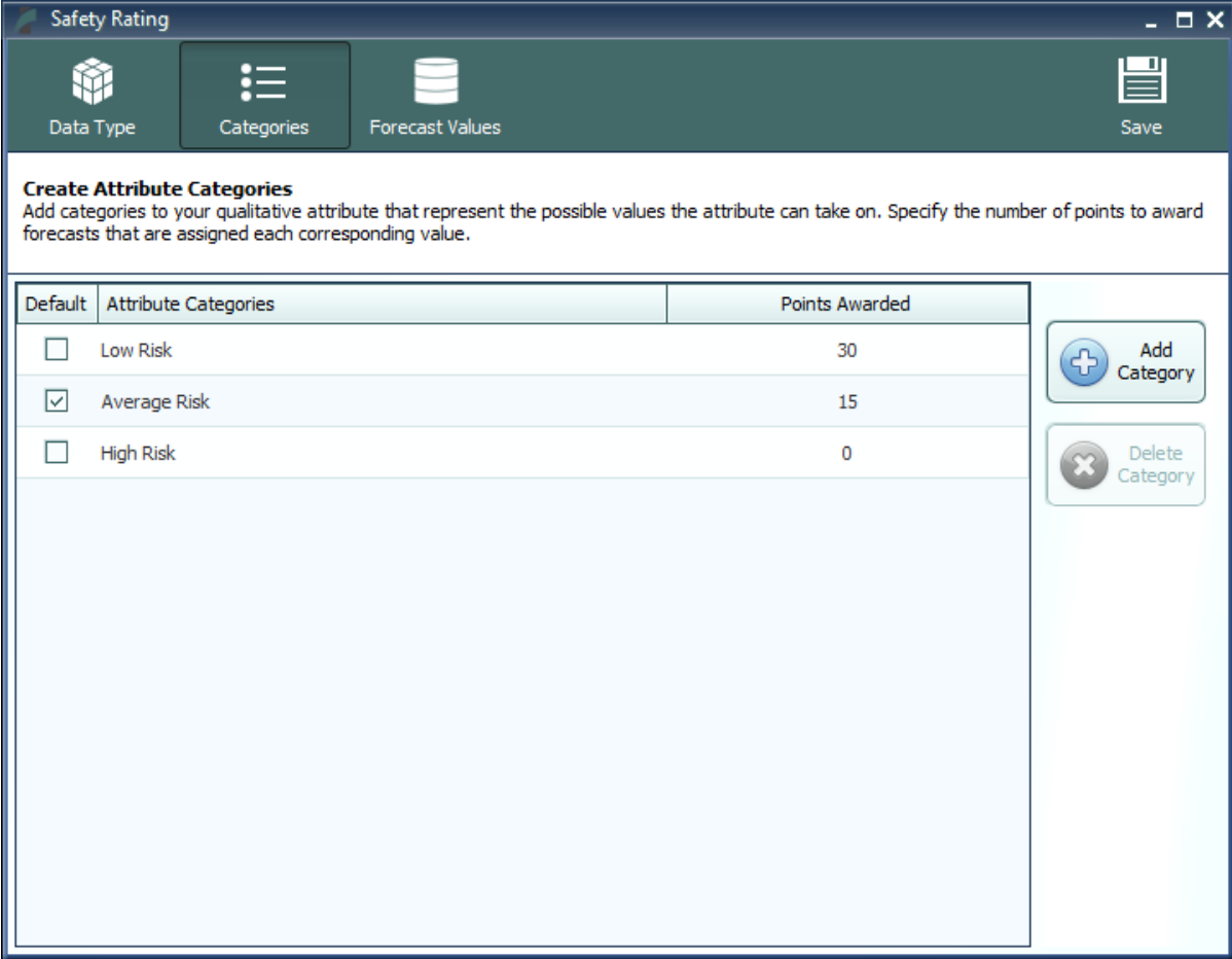
Figure 12: Attribute Score
