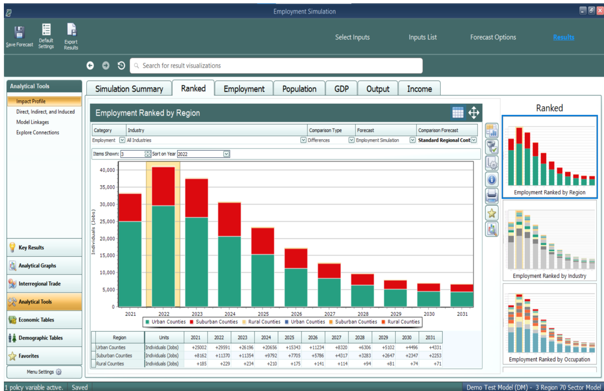
Figure 66: Ranked Visualizations
