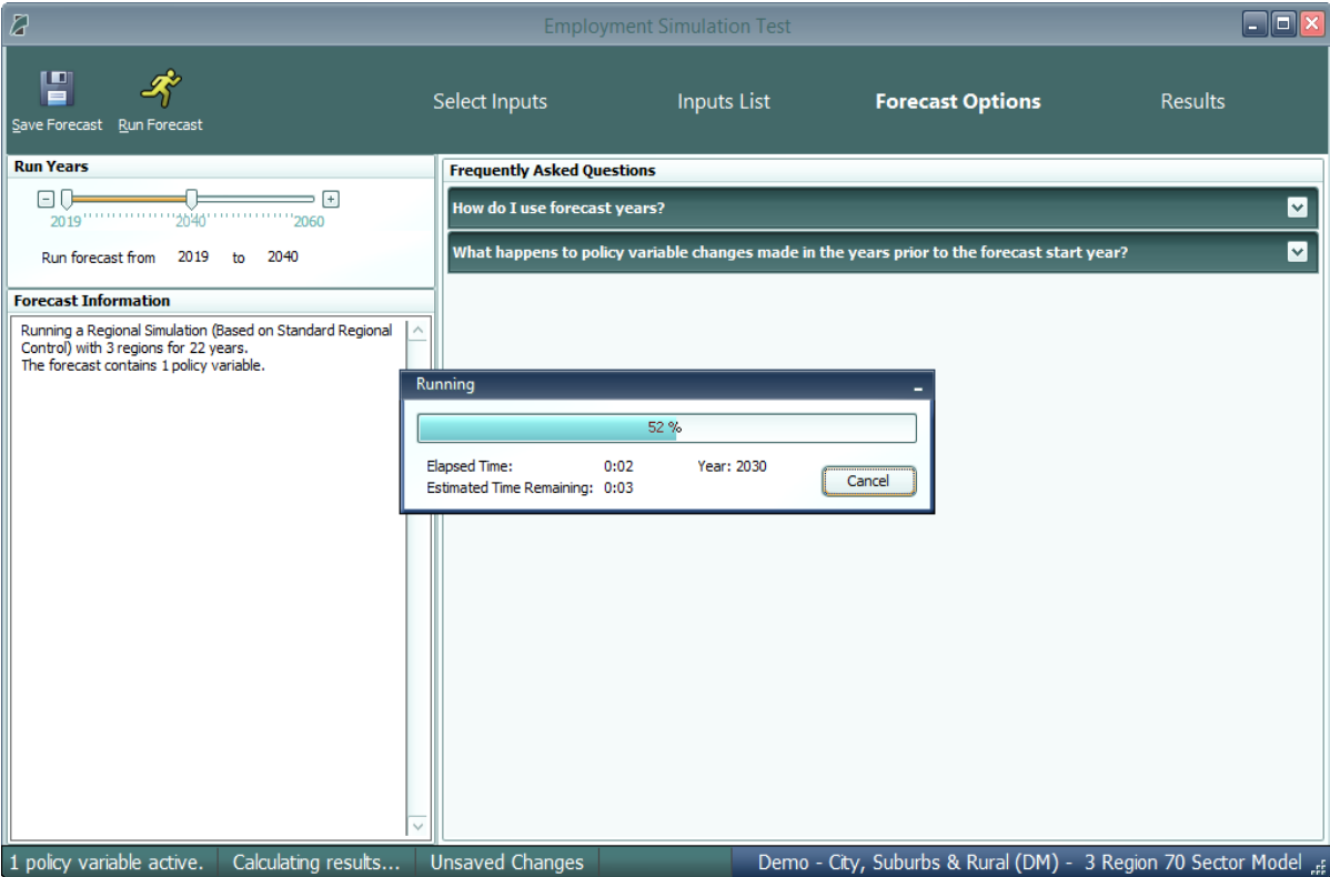
Figure 51: Forecast Options
