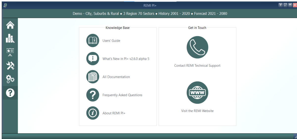
Figure 32: Help Center
