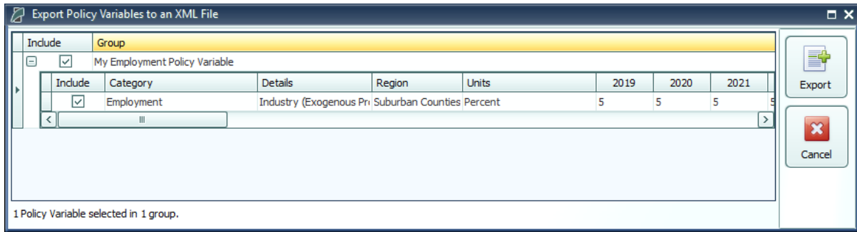
Figure 49: Export Center
