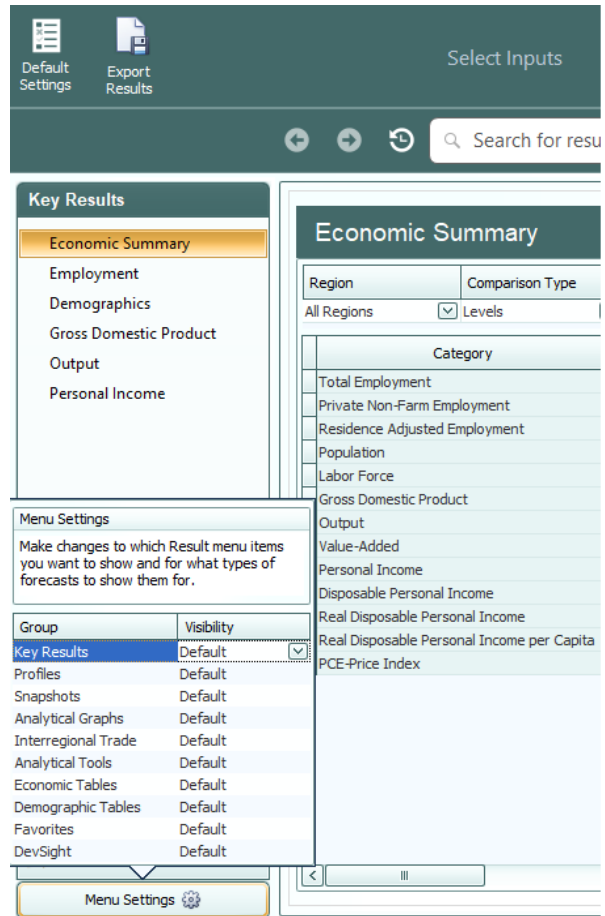
Figure 60: Menu Settings
