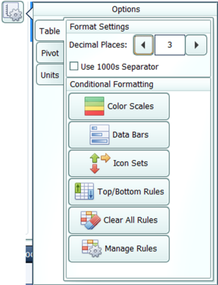
Figure 65: Conditional Formatting
