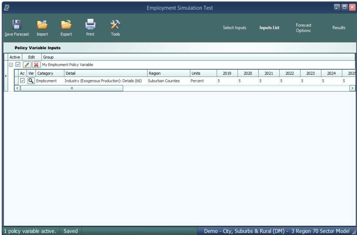
Figure 48: Inputs List
