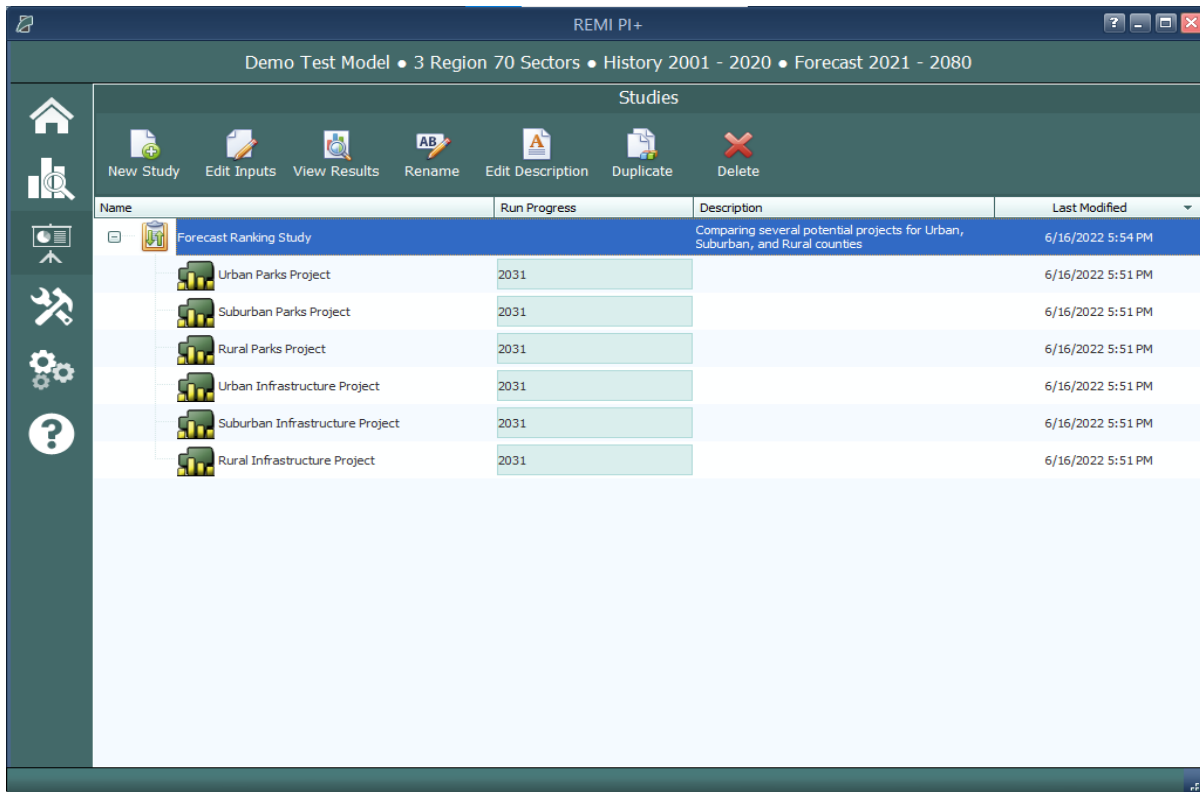
Figure 6: Studies List
