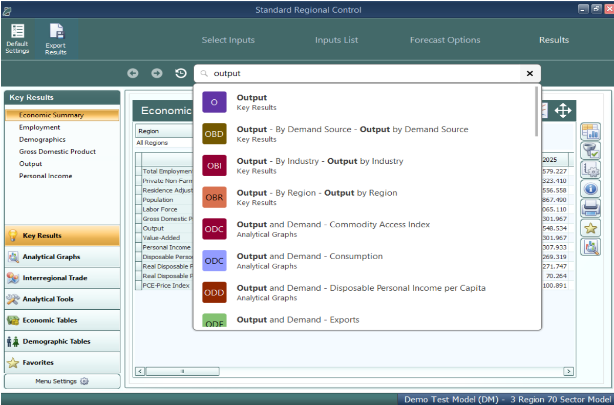
Figure 64: Results Search
