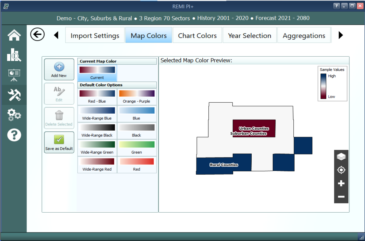
Figure 15: Map Colors
